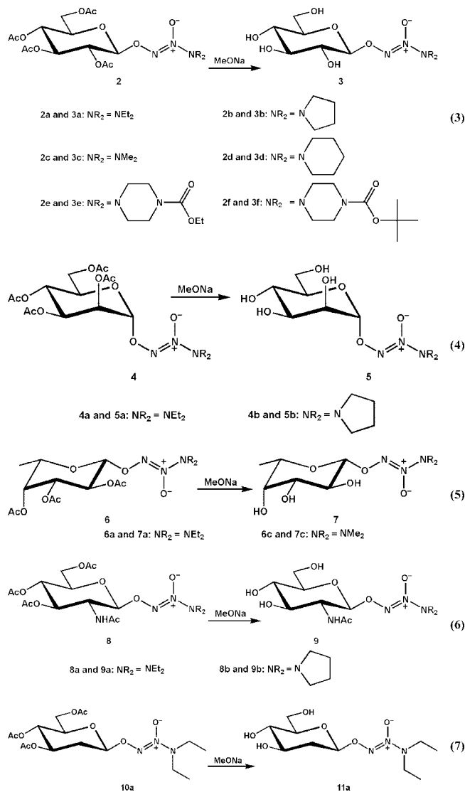
Scheme 2. General Synthesis of Glycosylated Diazeniumdiolates Described in This Work
