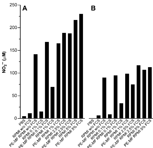
Figure 3. Generation of NO after parallel incubations of 9b at concentrations of (A) 250 and (B) 125 \mu M under different conditions. Substance 9b was incubated in phosphate-buffered saline (PBS) alone; RPMI cell culture medium without (w/o) or with addition of 0.1%, 1%, 2.5%, and 5% fetal calf serum (FCS) in the absence or presence of peritoneal exudate macrophages from iNOS-deficient mice (PE-MF); cultured in serum-free or serum-containing (0.1%, 1%, 2.5%, or 5% FCS) RPMI. Supernatants were harvested after 24 h, and cumulative NO release was estimated by determining its auto-oxidation product, nitrite ion, using the Griess assay. Data shown are mean values of triplicates. Standard deviations were <5%. The results confirm that the macrophages are capable of metabolizing 9b to NO and that the accelerating effect of serum on the hydrolysis of 9b is concentration-dependent. Shown are results from one of two identically designed experiments, which yielded comparable results.
