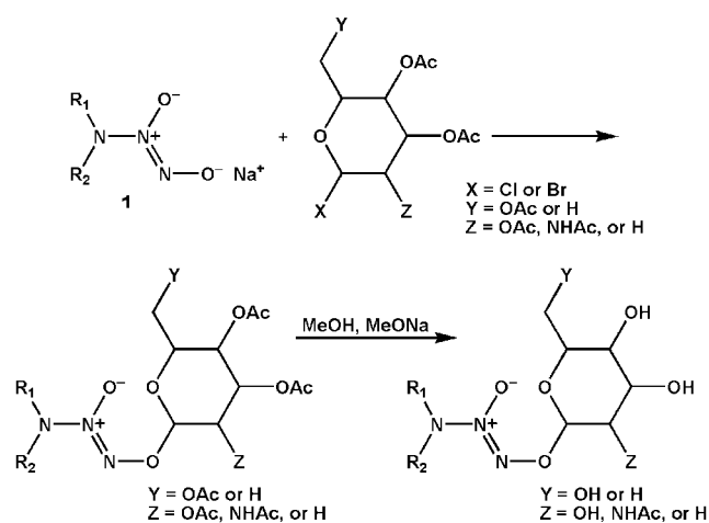
Scheme 2. General Synthesis of Glycosylated Diazeniumdiolates Described in This Work
