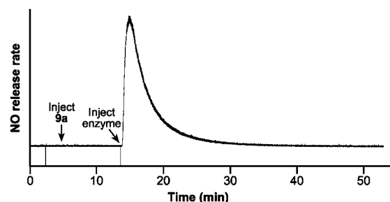
Figure 4. Chemiluminescence trace showing the time course of NO release from 0.39 \mu M 9a at 37 °C in 50 mM citrate buffer (pH 5.0) with 1.6 \mu g/mL of jack bean \beta -N-acetylglucosaminidase.
